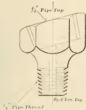
N. Y. A. B. CO. PLUG FOR FITTING OIL CUP TO 8" AND 9 1/2" AIR PUMPS.
